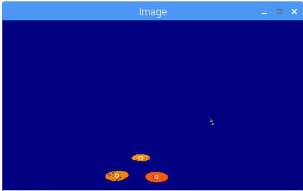
Figure 8 Image Segmentation
