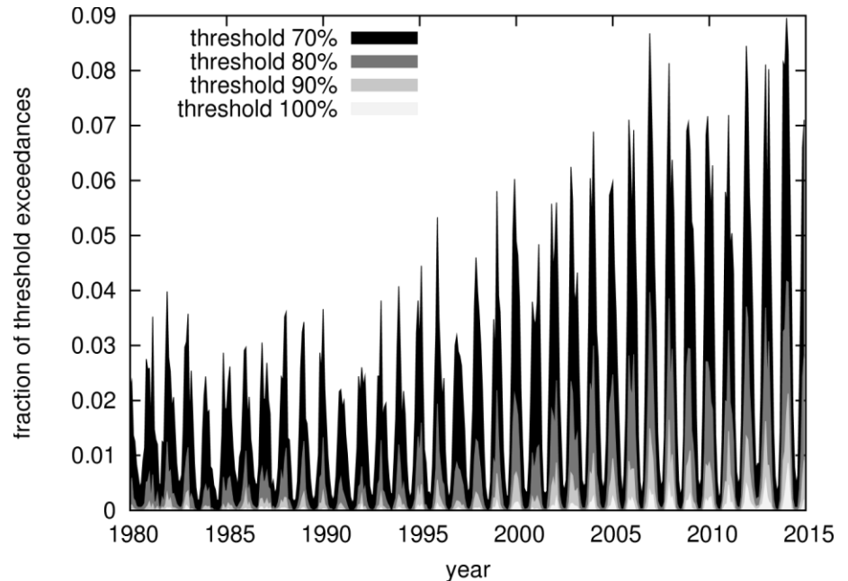
Figure 1. Time series of the fractional occurrence of high values of UTHi retrieved from HIRS channel 12 brightness temperatures in the northern midlatitude zone 30° to 70°. Use has been made of the data intercalibrated by Shi and Bates (2011). Note the strong increase that occurred with the transition from HIRS 2 to HIRS 3 around 1999.
