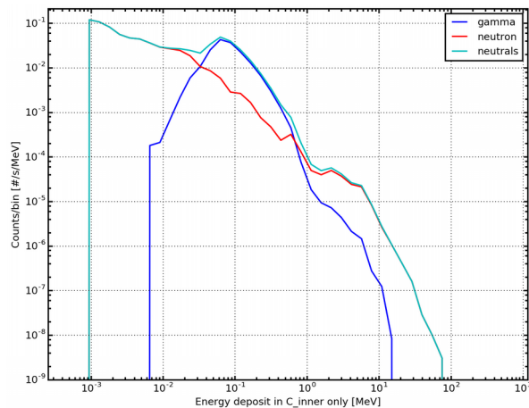
Fig. 3: Simulated neutron energy deposit spectrum in the inner segment of detector C.
