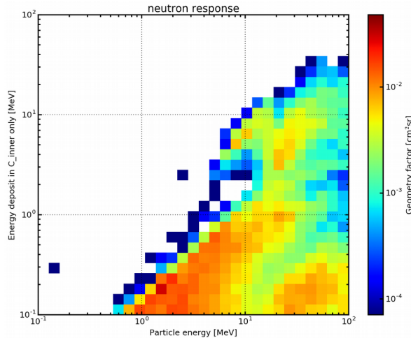
Fig. 2: LND instrument response function for fast neutrons serves as input for the inversion process which is needed to obtain the fast neutron spectrum.
