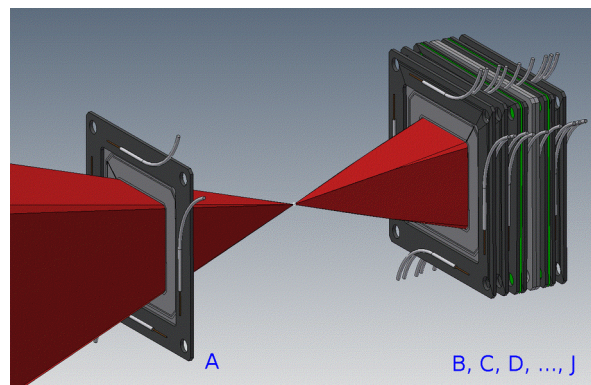
Fig. 1: LND measures charged particles with a stack of 10 Si solid-state detectors. A is the entrance detector on the left, B the first detector in the stack to the right. The following detectors (C,...,J) complete the stack.
