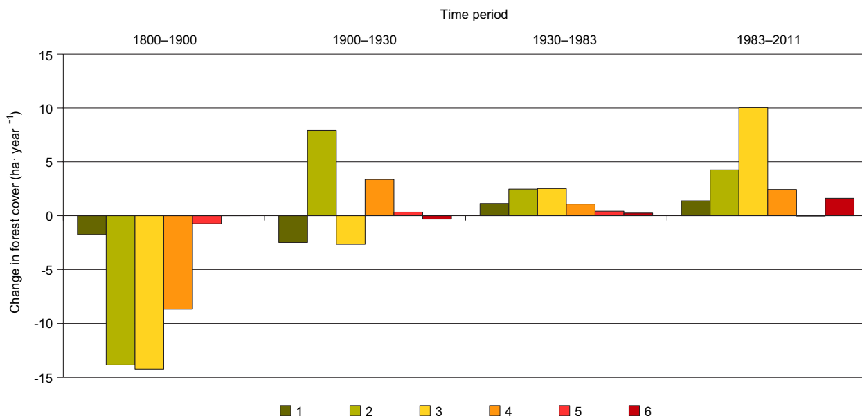
Fig. 5. Changes in the forest cover for selected soil types found in the Świętokrzyski National Park and its buffer zone since the year 1800 Soil types: 1 - sand-based, 2 - clay-based, 3 - loess-based, 4 - alluvial dust deposits, 5 - marshy and alluvial soils, 6 - rocky and skeletal soils.
