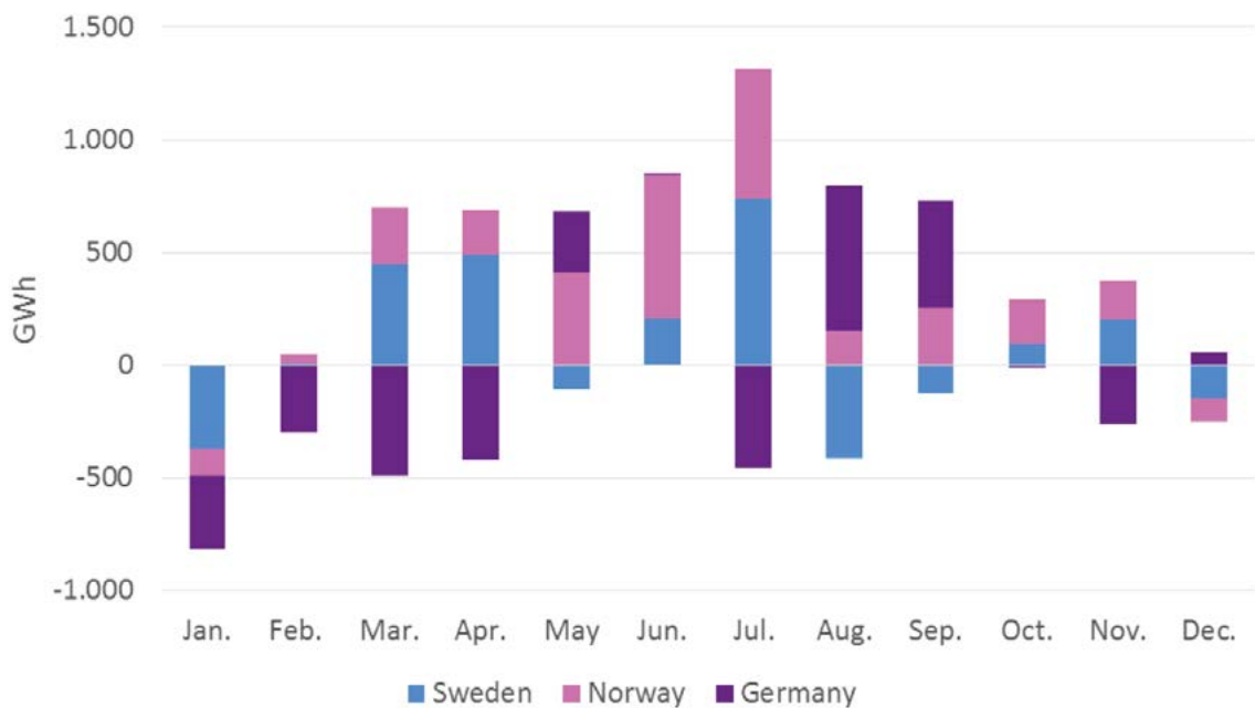
Figure 3: Import and export of electricity from Denmark to neighboring countries in 2014. Imports to Denmark from abroad are indicated by positive numbers. Exports from Denmark to abroad are indicated by negative values [13].
