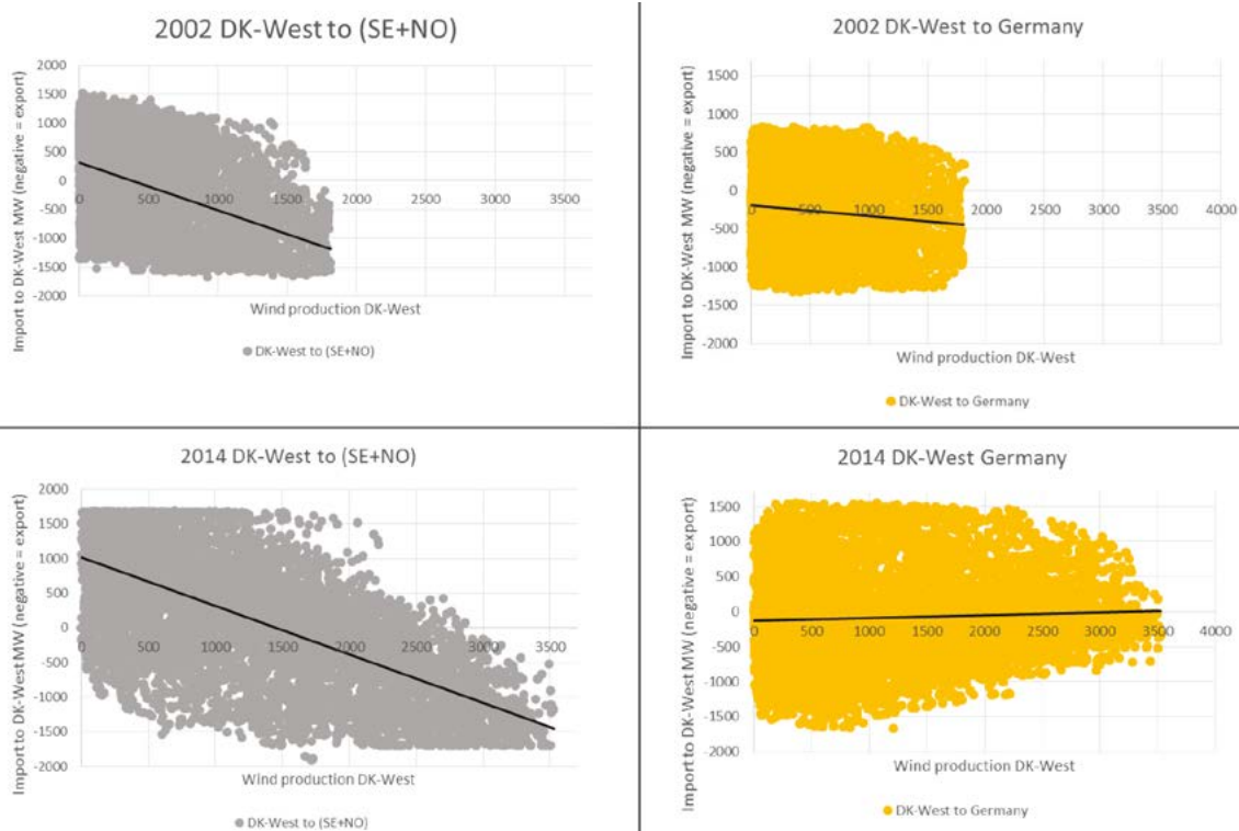
Figure 4: Correlation between wind power generation in West Denmark and flows to Sweden/Norway and Germany [1], p. 24.
