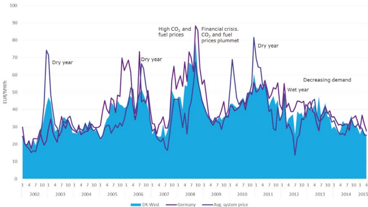
Figure 1: Spot market prices in Denmark between 1999 and 2014, based on [12] and [1], p. 22.
