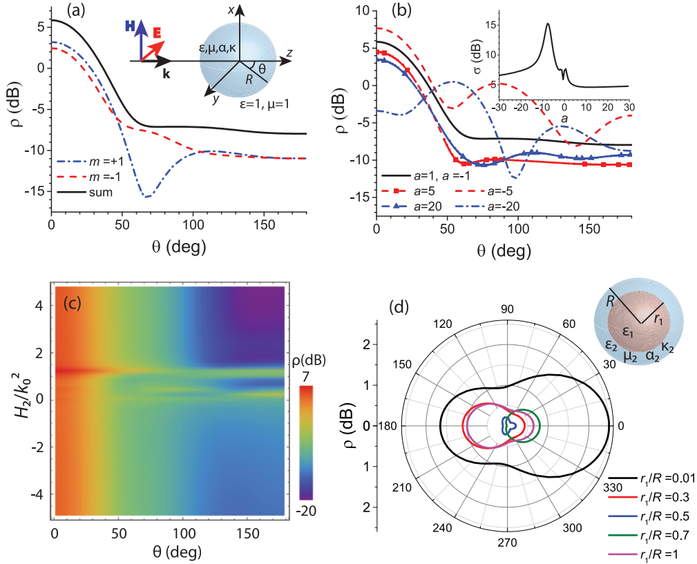
FIG. 1. Scattering cross-sections for the particles supporting Airy-exponential waves. (a) Chirality results in the distinct differential cross-sections \rho(\theta) for the right- and left-handed polarized waves [ m = \pm 1 in Eq. (B9)]. The inset sketches geometry of the scattering. Differential cross-section against parameters defining the inhomogeneous medium, quantities (b) a and (c) H_2 . The total cross-section is depicted in the inset in (b). (d) Variation of the differential scattering pattern depending on the radius of the core r_1 in the core-shell geometry (particle radius k_0 R = 1 and core permittivity \epsilon_1 = 3.5^2 ). Default parameters: a = 1 , g_1 = 1 + i , H_2/k_0^2 = H_3/k_0^3 = 1 , and k_0 R = \pi .
