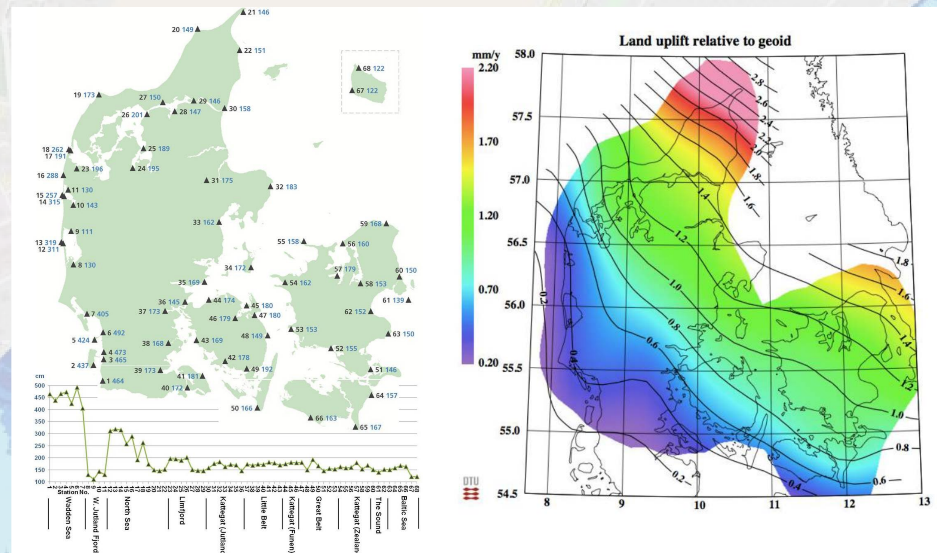
Figure 2: (left) 100 yr return heights (in blue) in cm above datum (DVR90) for 68 of the Danish water gauge stations (Sorensen et al., 2013), and (right) uplift rates in Denmark (Knudsen et al., 2016)
