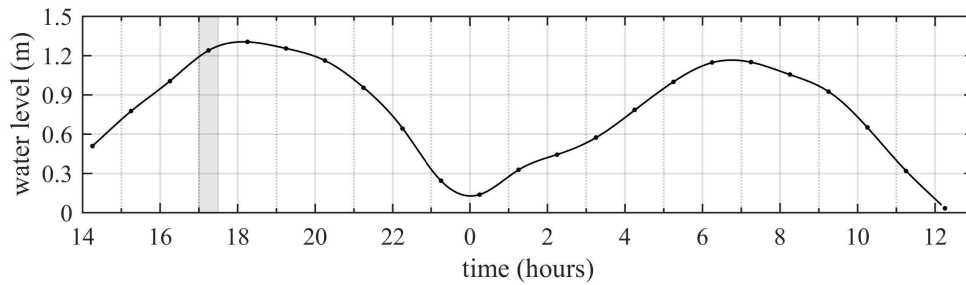
Figure 5. Water level above the pressure sensor showing the tidal variation during the field experiment. The time series start on September 21, 2016 at 14:00. The half-hour period marked in grey is used for detailed comparison between TCM and ADV below. See also wave energy spectrum for this particular interval in figure 4.
