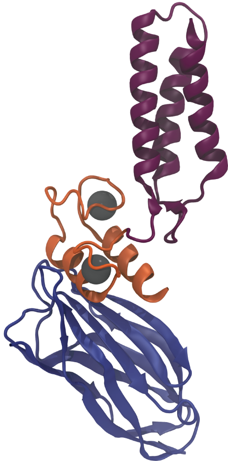
Figure 1. Crystal structure of the FIVAR-Doc : Coh complex (PDB accession: 2OZN, rendering in VMD 36 ). The three-helix bundle of FIVAR (purple) is fused to the Doc domain (orange) with its two calcium (grey spheres) binding loops and binds the immunoglobulin-like fold of the Coh (blue).
