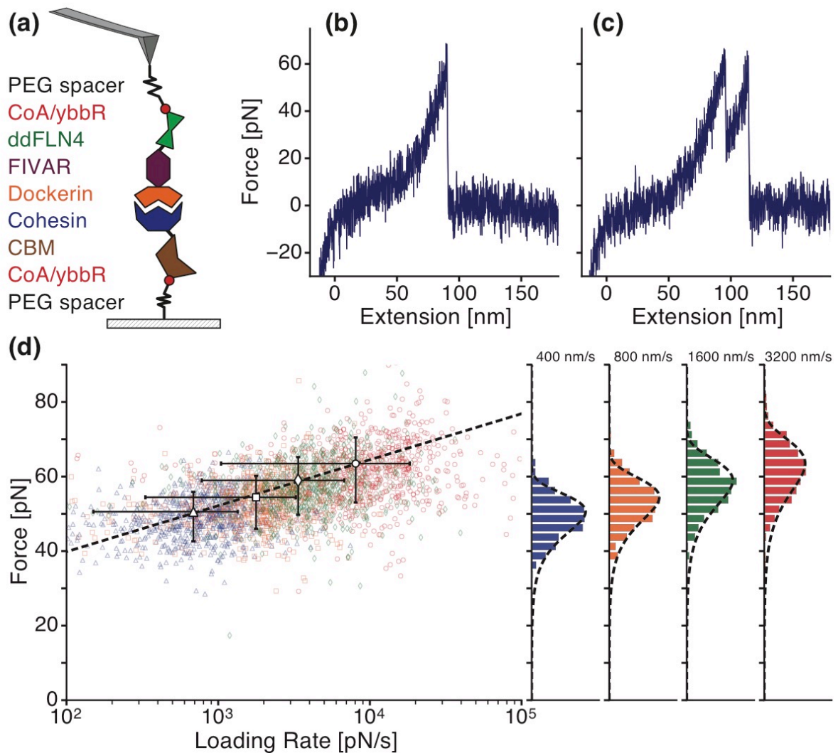
Figure 2. SMFS on the C. perfringens FIVAR-Doc : Coh complex. (a) Experimental setup with the ddFLN4-FIVAR-Doc immobilized on the cantilever and the Coh-CBM bound to the surface. A typical force-extension trace for a Coh-Doc complex rupture event without (b) and with (c) preceding unfolding of the FIVAR domain. (d) Dynamic force spectrum for Coh-Doc complex rupture with FIVAR unfolding as fingerprint. The respective pulling velocities were 400 nm/s (blue triangles), 800 nm/s (orange squares), 1600 nm/s (green diamonds), 3200 nm/s (red circles). The corresponding rupture force histograms and individual distribution fits (black dashed lines) are projected onto the right axes. The fit through the most probable rupture force and force loading rate (black, dashed line through white
