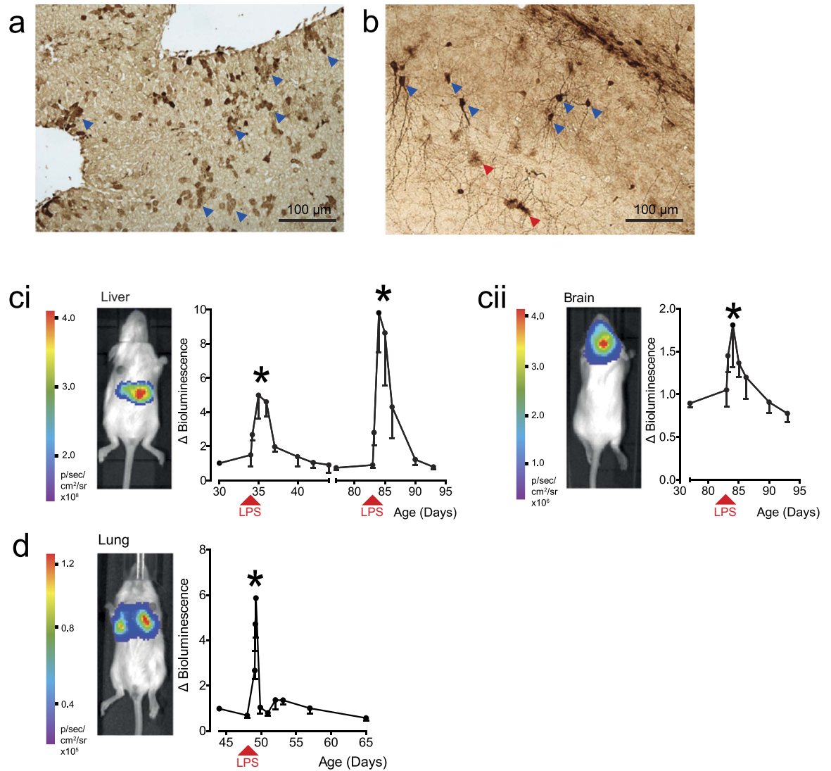
Figure 3. Lipopolysaccharide (LPS)-mediated induction of NF \kappa B-activated reporter cassette in targeted organs of reporter mice.
