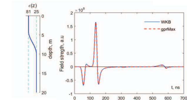
Fig. 2. Profile of half-space dielectric permittivity and simulated A-Scan.
