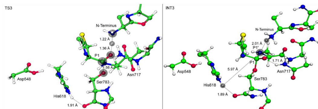
Figure 6. Representation of the structures of the transition state (TS3) and the intermediate (INT3) of the third step of the reaction.
