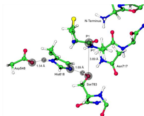
Figure 3. Structure of the reactants highlighting the most relevant distances for the first mechanistic step.
