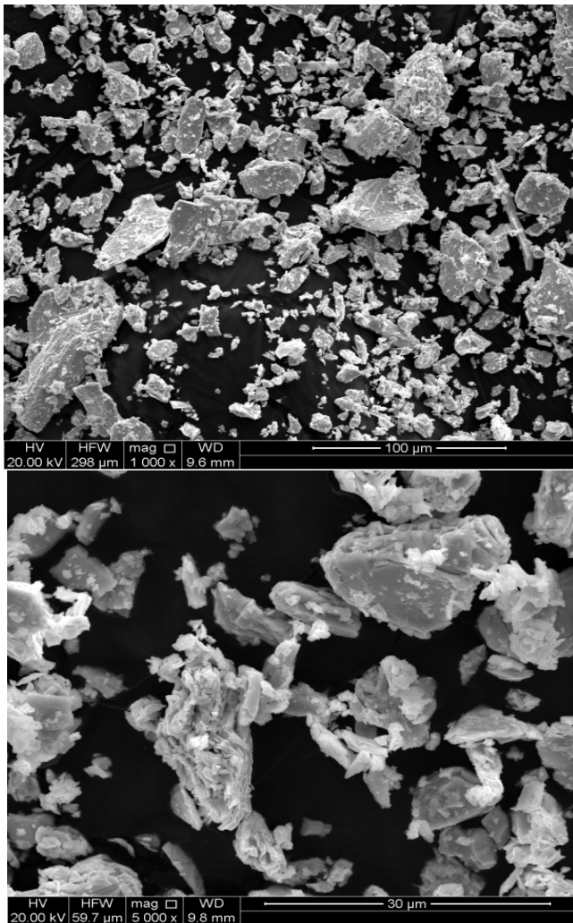
Fig. 2 The SEM image of p-type \text{Bi}_2\text{Te}_3 powder at diverse magnifications (1000x and 5000x)
