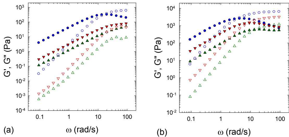
Figure 8. (a) Variation of storage modulus (hollow symbols) and loss modulus (filled symbols) of P(DMA-N1) solutions ( C_p=10 wt% (left) and 20 wt% (right)) at T=5 °C as a function of added BB: B/N=0.5 ( \triangle , \blacktriangle ); 1 ( \circ , \bullet ) and 1.5 ( \nabla , \blacktriangledown ).
