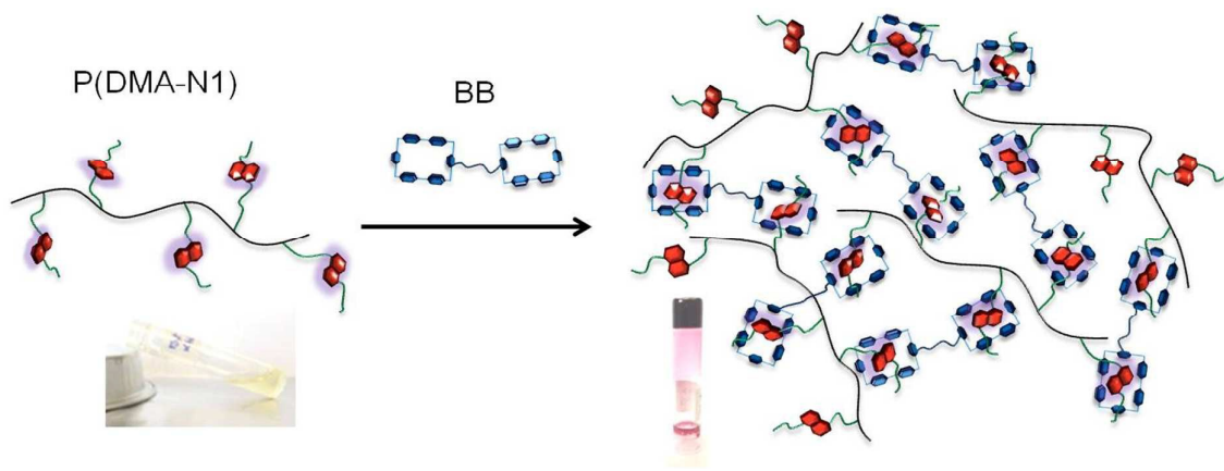
Figure 1. Formation of a supramolecular polymer network induced by host-guest interactions
