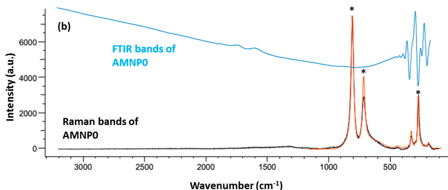
Figure 2. Raman and FTIR spectra of (a) Alfa Aesar tungsten carbide WC and (b) AMNP0. Spectra in red show reference Raman bands associate with related tungsten compounds. Symbols * denote the optimal vibrational Raman peaks observed at 803, 715 and 265 \text{cm}^{-1} .
