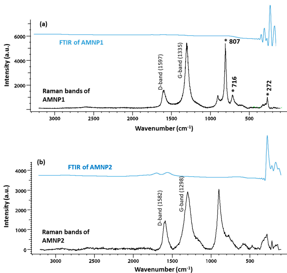
Figure 3. Raman and FTIR spectra of (a) AMNP1 and (b) AMNP2.
