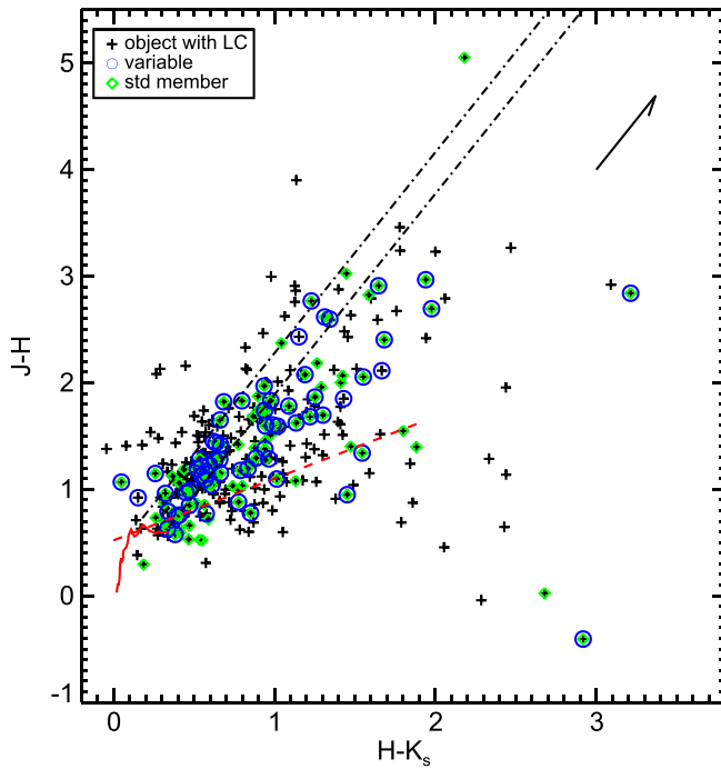
Figure 8. J - H , H - K_s for objects with light curves in the catalog, with variables and the standard set of members indicated as shown. (The right panel is a zoom-in on the densest region from the left.) The red solid line is the expected ZAMS location; the red dashed line is the classical T Tauri locus from Meyer et al. (1997). A reddening vector for A_V = 6 is shown; the black dotted-dashed line are extensions of the ZAMS according to this reddening law. This plot suggests that there is not a large contamination rate from foreground/background sources; see text.
