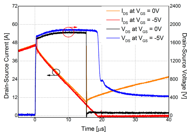
Figure 4. Experimental V_{DS} and I_D waveform; I_{AV} \sim 47 A; V_{DD} = 400 V; T_{CASE} = 25 °C; V_{GS} = 0 V and -5 V; L = 500 \mu H (Comparison).
