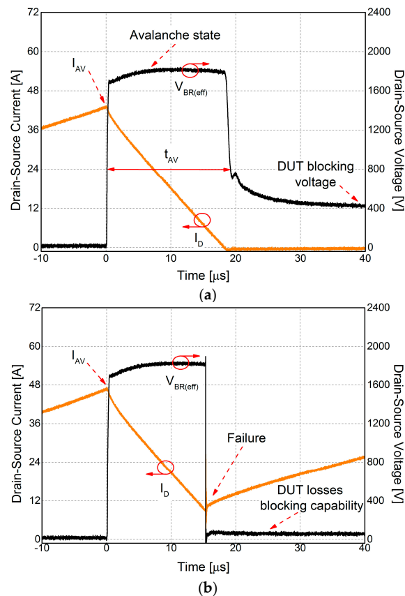
Figure 3. Experimental V_{DS} and I_D waveform; V_{DD} = 400 V; T_{CASE} = 25 °C; V_{GS} = 0 V; L = 500 \mu H. (a) Without Failure; I_{AV} \sim 42 A; (b) At Failure; I_{AV} \sim 47 A.
