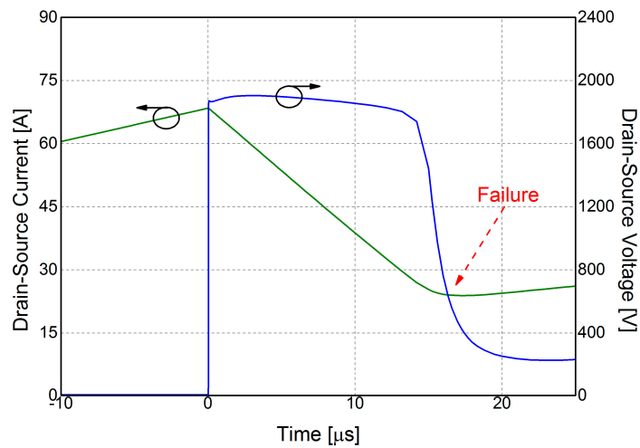
Figure 7. Simulated V_{DS} and I_D waveform— V_{DD} = 400 V; T_{CASE} = 25 °C; L = 500 μH.
