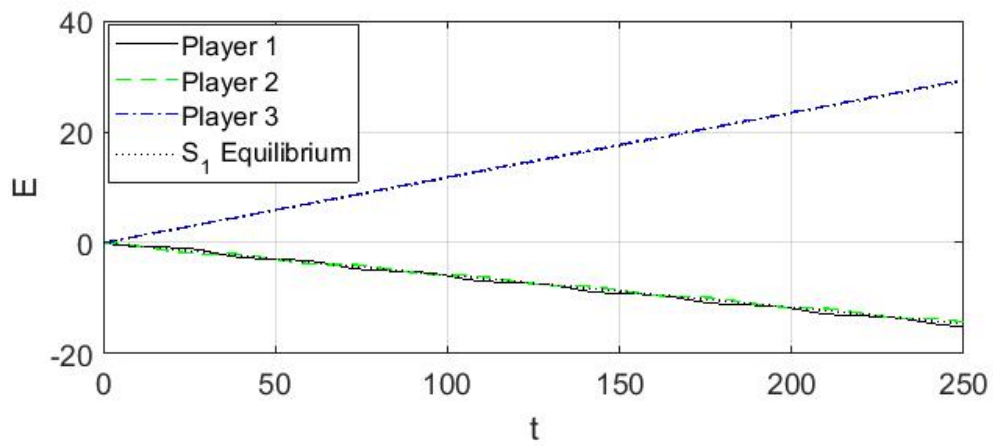
Figure 10: The ex-showdown expectations of the solutions shown in Figure 9.
