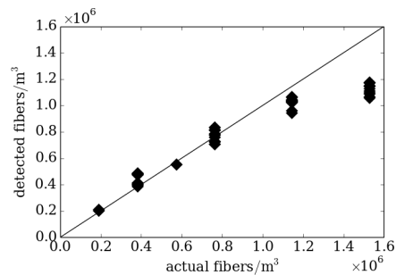
Fig. 10. Results of applying the fiber detection process to 64^3\text{mm}^3 data volumes containing a range of different fiber counts (from 190730 fibers/ \text{m}^3 to 1907300 fibers/ \text{m}^3 ). Each fiber is approximately 1mm in diameter and each voxel is 0.5\text{mm}^3 in size. The solid line represents the ideal, illustrating the number of fibers are correctly detected up to 1 \times 10^6 fibers/ \text{m}^3 .
