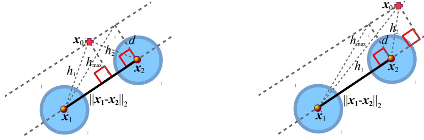
Fig. 3. Illustration of the geometry involved in the calculation of the distance from the line segment, d_{ls} . When h_1, h_2 \leq h_{max} (left) then d_{ls} = d . When h_1 or h_2 \geq h_{max} (right) then d_{ls} = \min(h_1, h_2) .
