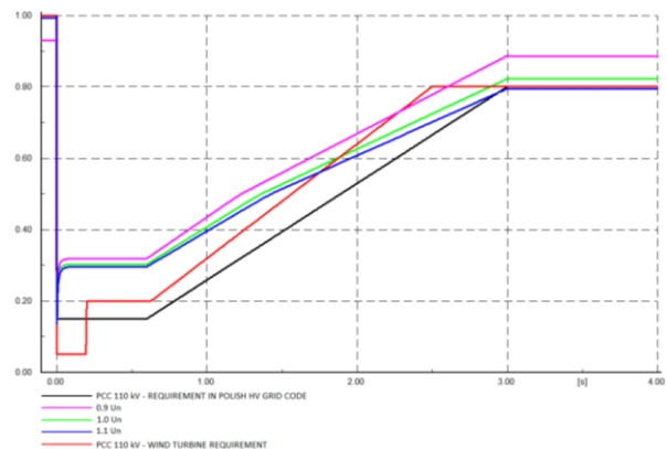
Figure 6: Wind turbine voltage characteristics during fault for different grid voltage levels
