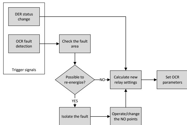
Figure 9: The adaptive algorithm
