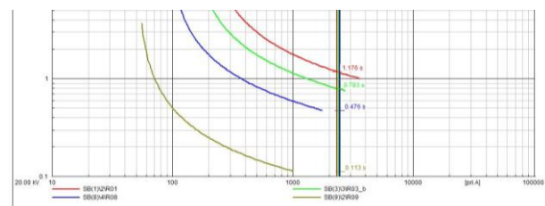
Figure 11: Relay operating times (adaptive settings)
