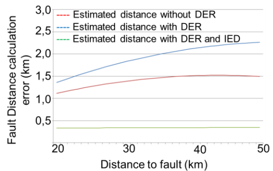
Figure 12: Fault distance algorithm error
