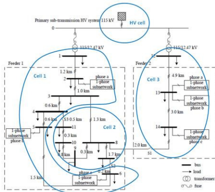
Figure 4: CIGRE MV model
