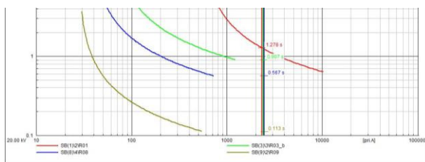
Figure 10: Relay operating times (static settings)
