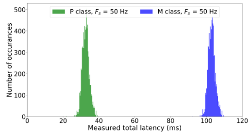
Figure 8: PMU WAN latency results
