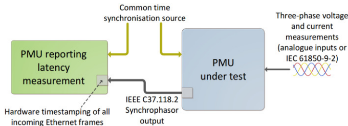
Figure 7: Overview of PMU reporting latency measurement method
