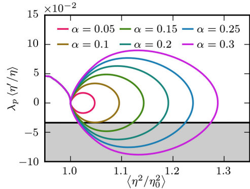
FIG. 3. Variation of the average plasma density gradient for the density profile (1) with \alpha \in [0.05, 0.3] . The region for which self-injection can occur, as described by (6), is shaded grey. \Gamma_e = 6 corresponding to a_0 = 4 .
