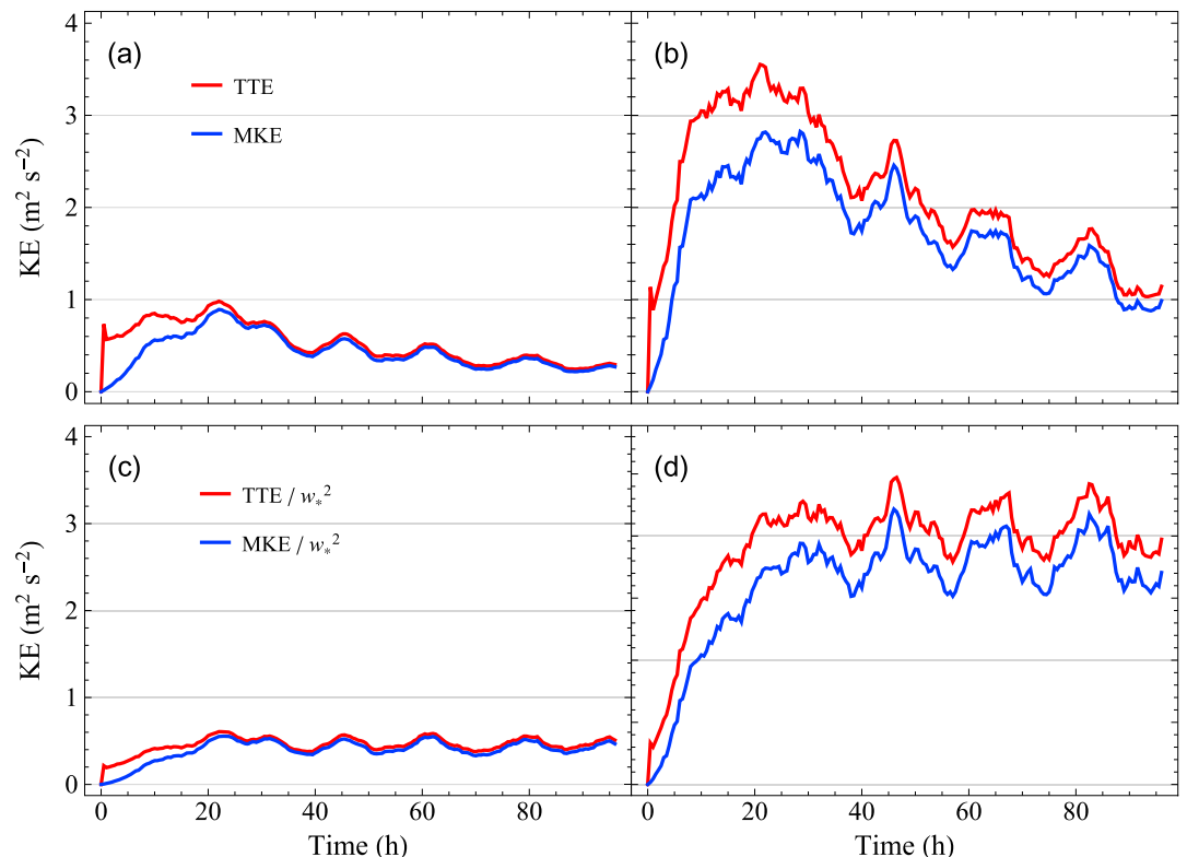
Figure 4. The temporal evolution of domain-averaged kinetic energies. (a and c) Rural area. (b and d) Urban area. Figures 4a and 4b show the original values, while Figures 4c and 4d show the normalized values.
