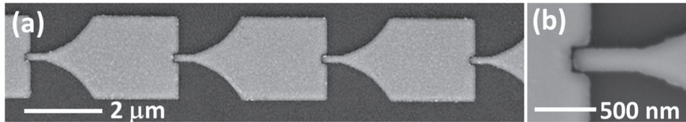
Figure 2. (a) SEM image of a chain of elements forming part of the shift register. (b) Close up showing the narrow spacing between the wire and square element.
