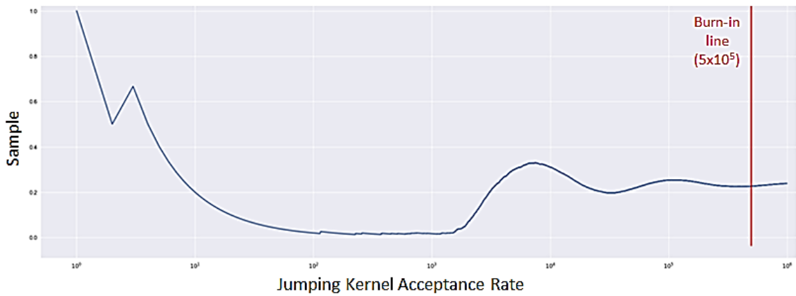
Figure 20. No grouping scheme data set 6 a) jumping kernel variance and b) MCMC acceptance rate
