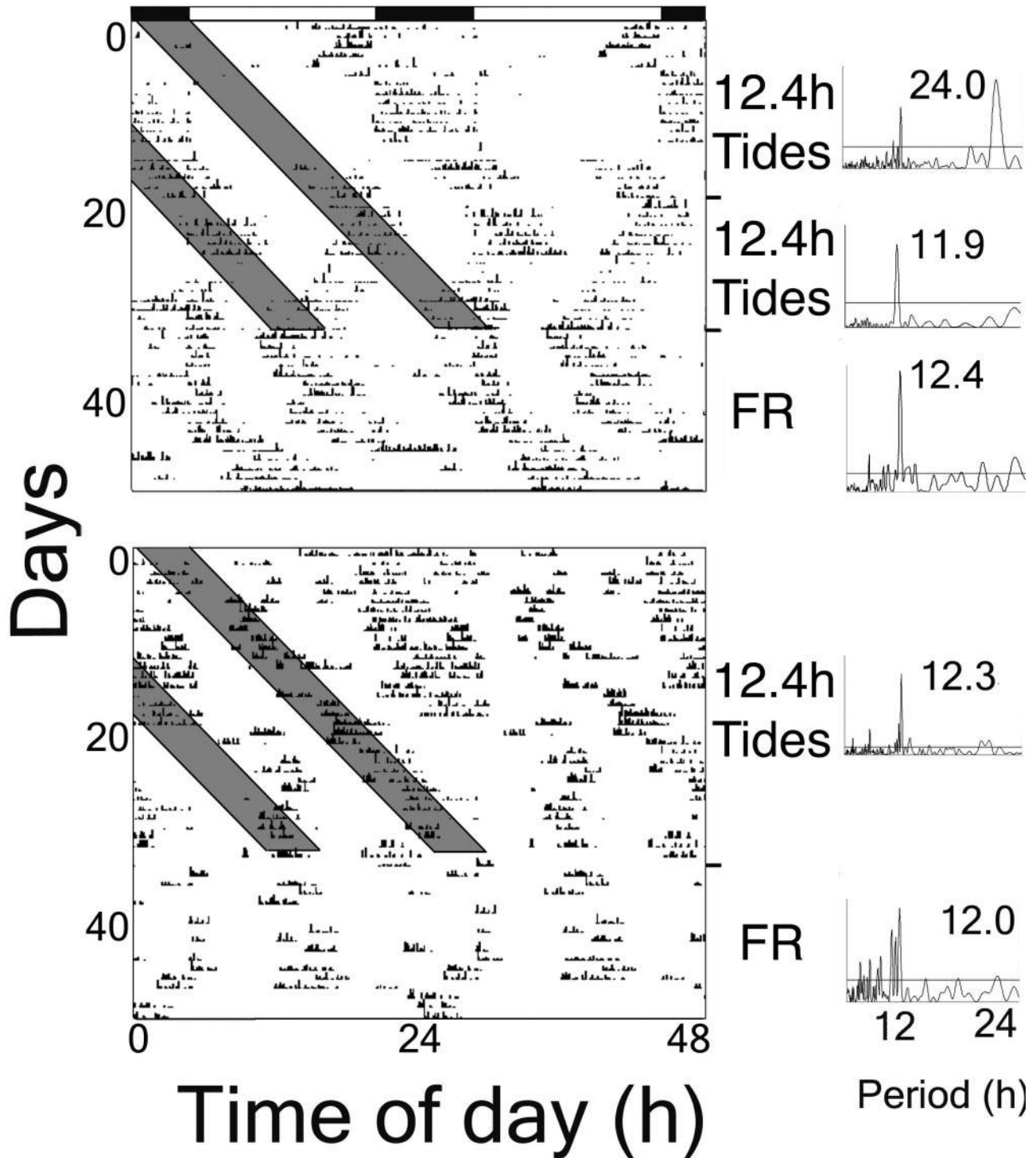
Figure 4. Entrainment of tidal rhythms by artificial tides. Two periodograms are shown in the top panel for the 12.4-h tide period to illustrate a significant change in tau over time. Experimental conditions as described for Fig. 3.
