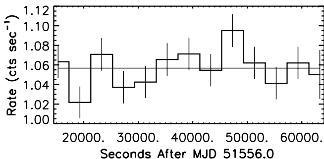
FIG. 2.—X-ray light curve of \delta Ori resulting from binning the valid events in all nonzeroth orders (the zeroth-order counts are ignored to avoid problems with photon pileup effects). The errors reflect Poisson statistics on the count numbers in each 4 ks bin. The horizontal line shows the mean count rate of 1.056 counts s^{-1} .
