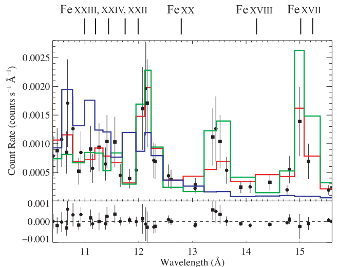
Figure 10. The binned MEG spectrum (squares are -1 order and circles +1 order) is shown along with the best-fitting (MEG -1 order) model (red). Cooler (0.3 keV, green), and hotter (1.5 keV, blue) models are also shown, making it clear that the presence of Fe XVII emission near 15 Å in the data and the low levels of emission near 11 Å from higher ionization stages are incompatible with very hot ( kT > 1 \text{ keV} ) plasma from CWS. Ne IX and Ne X emission complexes are also visible at 13.5 and 12.1 Å, respectively. Their ratio is temperature-dependent and consistent with temperatures between 0.3 and 0.6 keV. We indicate the wavelengths of some of the strongest lines at low and at high temperatures. Note that there are other, low-temperature lines of, for example, Ne IX contributing to the observed flux in the short-wavelength side of the spectral region displayed in this figure.
