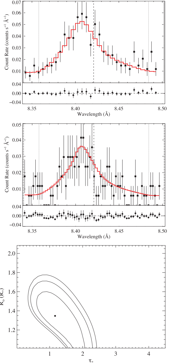
Figure 7. The derived value of \tau_* is also low for the Mg XII Ly \alpha line at 8.421 Å shown here, but it is modestly higher than the shorter wavelength Si XIII complex shown in the previous figure.
