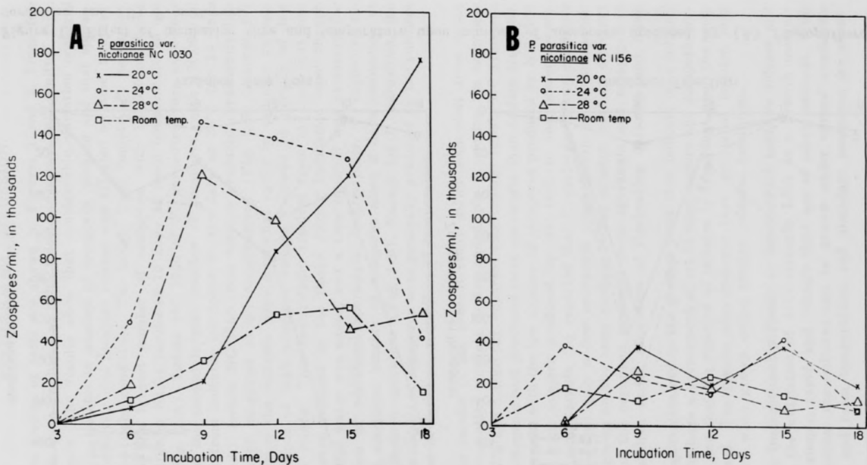
Figure 2. Effect of incubation time and temperature upon number of zoospores produced by (A) Phytophthora parasitica var. nicotianae NC 1030, and (B) P. parasitica var. nicotianae NC 1156.
