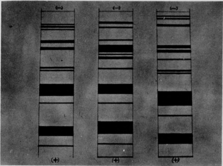
Fig. 5. Electrophoreograms Of Three Modenas.
