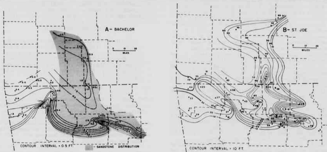
Figure 1. Isopachous maps of the Bachelor (A) and St. Joe (B) Formations, northern Arkansas and southwestern Missouri (data from Thompson and Fellows 1970, McFarland 1975b, and Shanks 1976).
