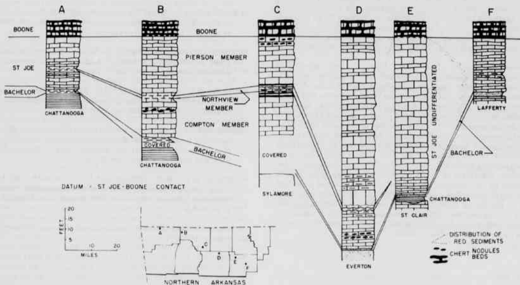
Figure 2. Correlation of selected sections of lower Mississippian strata in northern Arkansas (data from Thompson and Fellows 1970, McFarland 1975b, and Shanks 1976).
