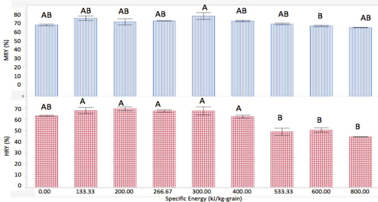
Figure 4.2: Effect of increasing microwave specific energy on the milled rice yield and head rice yield of medium grain rice. Means with the same type of letters are not significantly different at \alpha = 0.05 .
