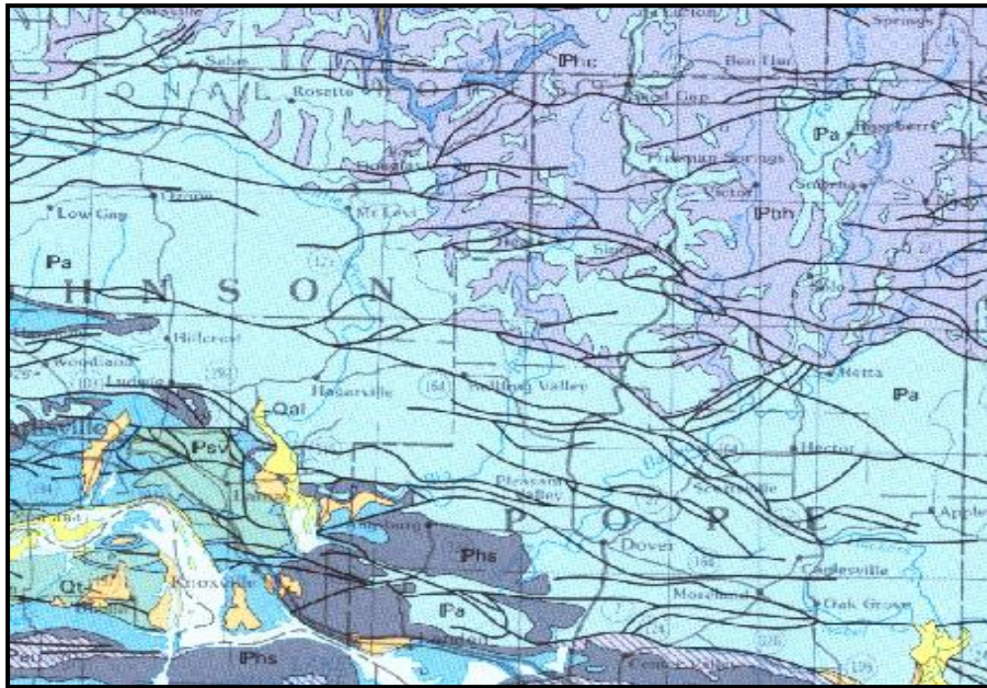
Figure 3-5: The geological map of the study area, depicting the regional east- west trending faults (modified from Arkansas Geological Survey).
