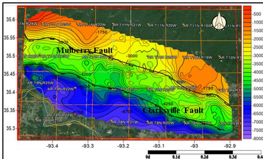
Figure 3-6: Structural contour map of the Hale Formation interval.
