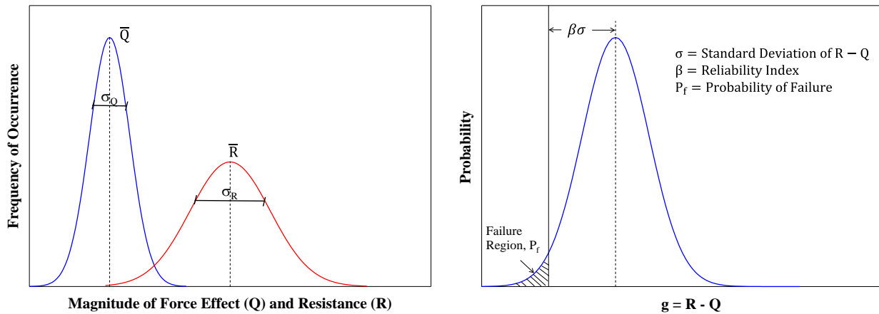
Figure 1.1. a) Force and resistance frequency distribution and b) probability distribution of the difference in the resistance and applied forces (modified from Brown et al. 2010).
