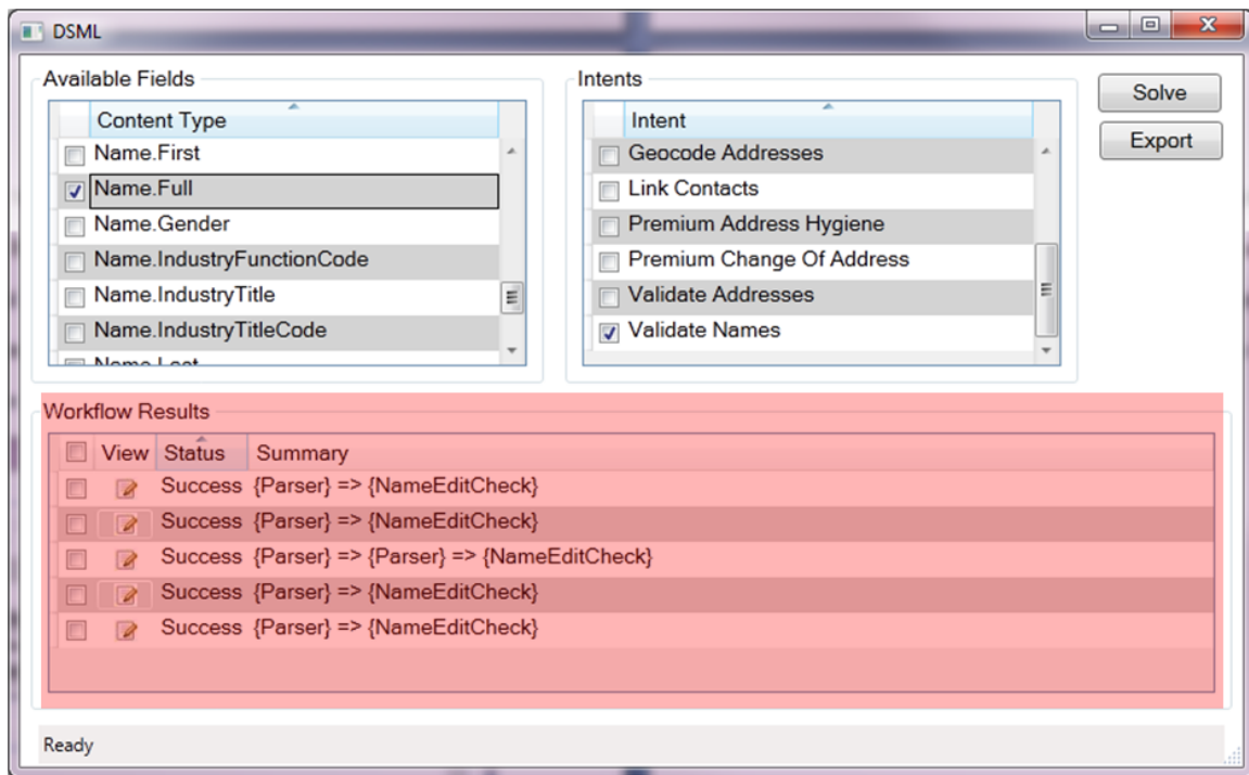
Figure 27: Workflow results in GUI.
