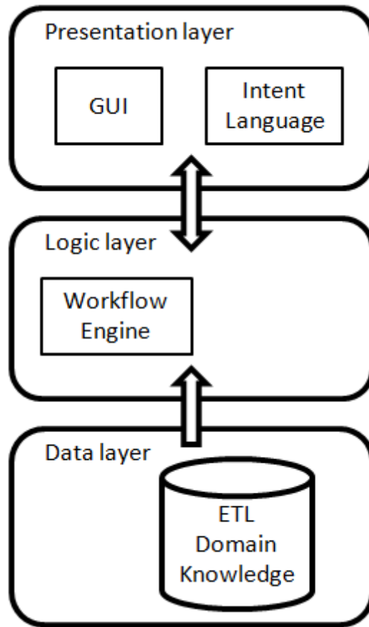
Figure 19: High-level architecture of the prototype.
