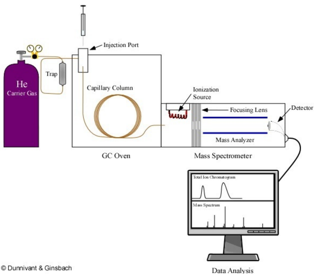
Figure 1.3 A simplified model of a gas chromatograph mass spectrometer. Reproduced from Dunnivant and Ginsbach, 2008.
