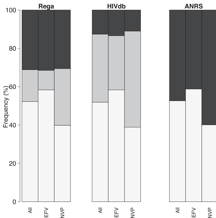
FIG. 2. Genotypic resistance scores for rilpivirine in different patient populations. ALL, all patients (n = 1212); EFV, efavirenz-experienced (n = 813); NVP, nevirapine-experienced (n = 399). For each interpretation algorithm, proportion of patients scored as high-level resistant (dark grey), intermediate resistant (grey) and susceptible (light grey).
