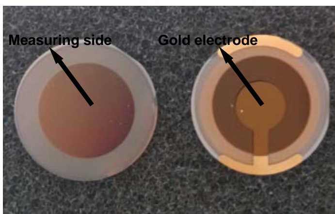
Figure 5: Both sides of the quartz-crystal.
