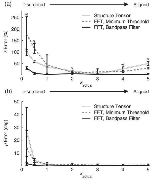
Fig. 5 Comparison of image analysis methods. (a) Error in measuring k and (b) error in measuring \mu when fiber networks vary from disordered to aligned. Bars represent standard deviation (* p < 0.05 )
