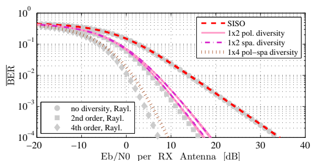
Fig. 4: Measured BER characteristics for uncoded 4-QAM modulation with equal channel gains (after path loss removal)
