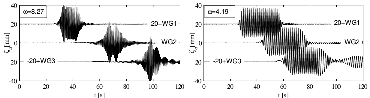
Figure 4 Wave records at WG1 , WG2 and WG3 , for a wave height H = 30 \text{ mm}
