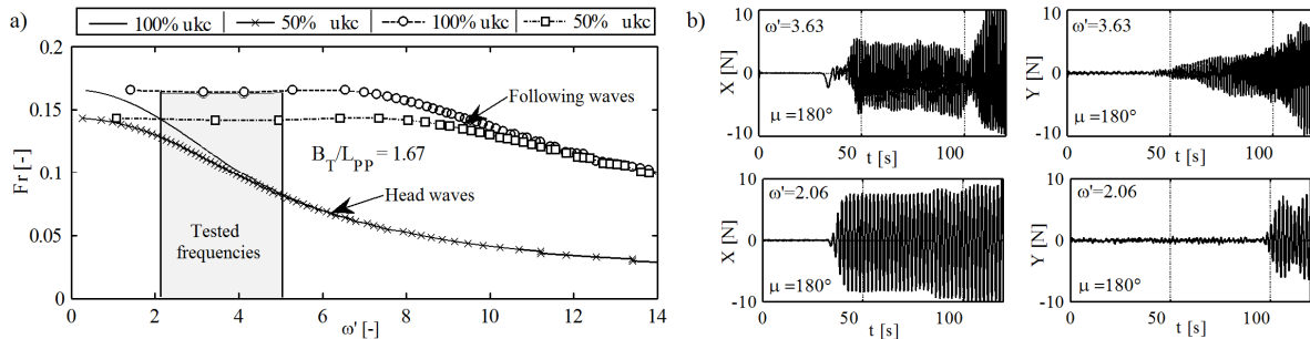
Figure 7 (a) Critical speed for the ship COW, and (b) measured surge and sway forces at zero speed, 100% ukc , \omega' = 3.63 , \zeta_a = 32.8 mm (top) and \omega' = 2.06 , \zeta_a = 10.1 mm (bottom)
