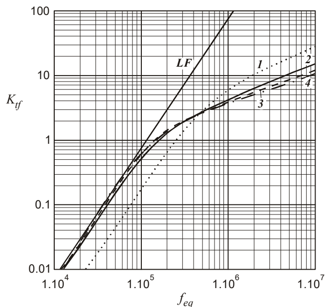
Fig. 1. Typical transformer factor K_{jf} for d = 0.5 mm, \rho_c = 23 \cdot 10^{-9} \Omega \cdot m and \lambda = 0.5 at \eta = 0.9 ; 1) dotted line: half layer, m_E = 0.5 ; 2) solid line: single layer, m_E = 1 ; 3) dashed: two layers, m_E = 2 ; 4) dash-dot: three or more layers, m_E > 2 . LF— low frequency approximation.
