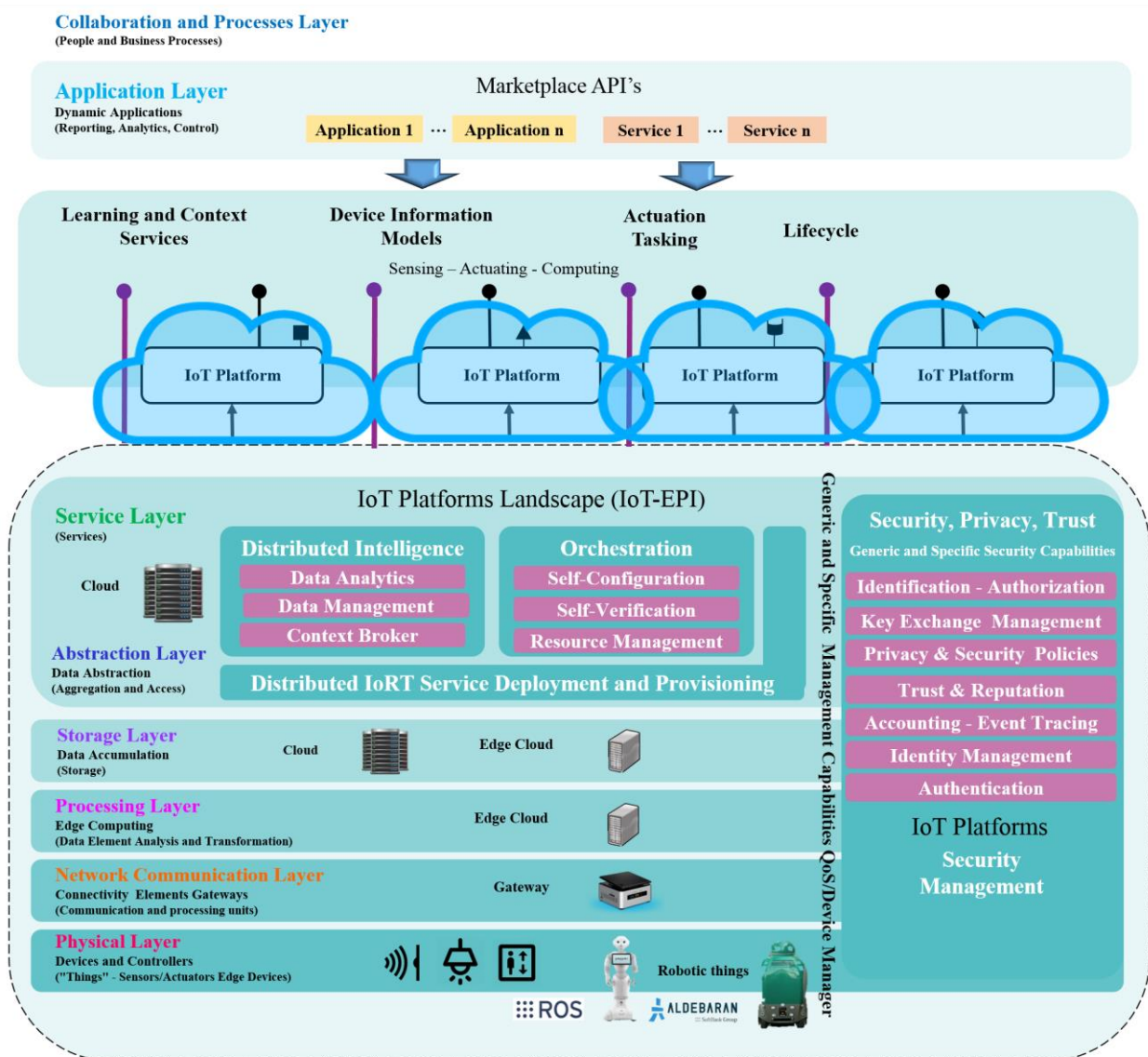
Figure 4.8. IoRT layered architecture
