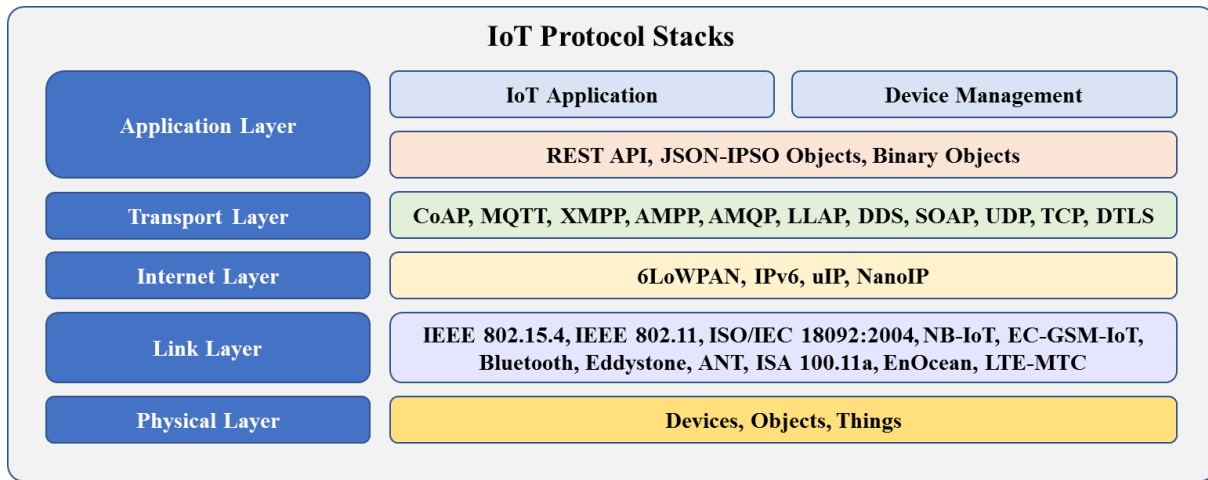
Figure 4.2. Communication protocols used by different IoRT applications
