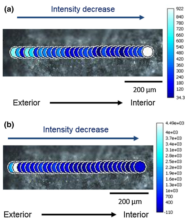
Fig. 5 Raman spectroscopy line scan from exterior (l of figure) to interior of the dark blue tesserae with integrated Raman band results from a 146 to 127 cm -1 and b 498 to 464 cm -1
