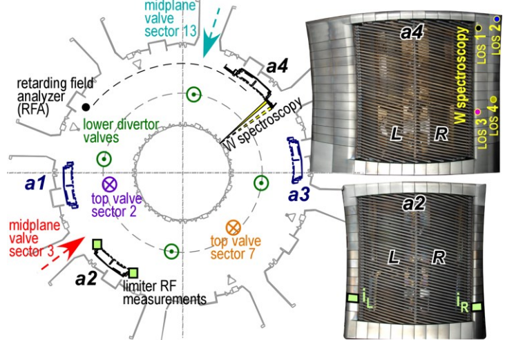
FIGURE 1. AUG toroidal view of ICRF antennas, gas valves and special diagnostics.
