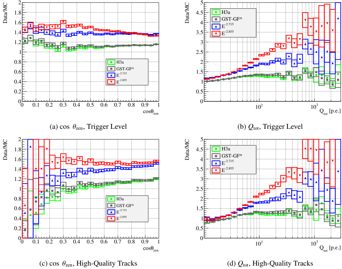
Figure 8: Ratio of experimental data to simulation in terms of reconstructed zenith angle \theta_{zen} and total amount of registered photo-electrons Q_{tot} . The primary flux models used in this comparison are discussed in Section 4.2.
