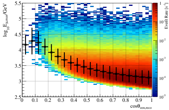
(a) Muon Surface Energy
