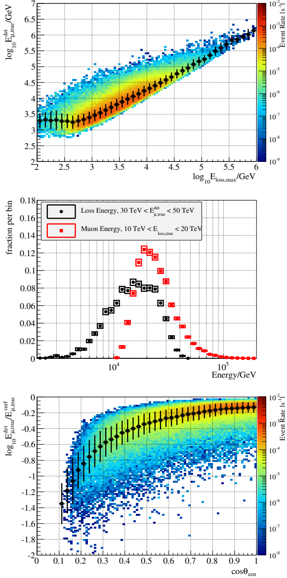
Figure 20: Top: Relation between most energetic single energy loss and leading muon energy within the Ice-Cube detector volume. Middle: Distribution of true energy parameters for two slices in top histogram. Bottom: Fraction of muon surface energy remaining at point of entry into detector volume in dependence of zenith angle. Figures are based on simulated events with primary flux weighted to E^{-2.7} power law spectrum and correspond to final analysis sample before application of minimum shower energy criterion. The black curves represent mean and spread of the distribution.
