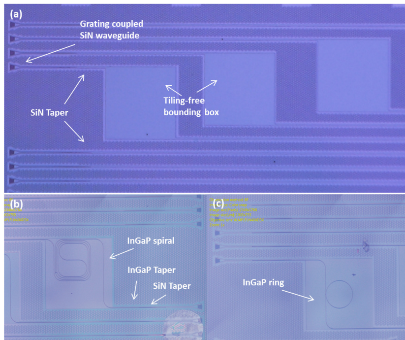
Figure 5.14 (a) The designed SiN chip with grating coupled waveguides connected to the SiN taper which will be used to coupled light to an InGaP taper fabricated on top of it. The InGaP taper can then be connected to a waveguide that leads to any desired device (which is on top of the bounding box). The bounding box has no tiling or any other SiN structures in it so that the InGaP device on top essentially feels the same refractive index environment as it would have in the InGaP-on-insulator platform. As such, the SiN chip can be used as a means of coupling in and out the light from the nonlinear devices in the InGaP-on-insulator platform. The final result of the fabrication process outlined in sec. 5.2 resulting in devices such as (b) an InGaP spiral and, (c) an InGaP ring resonator coupled to the SiN via inverted tapers.
