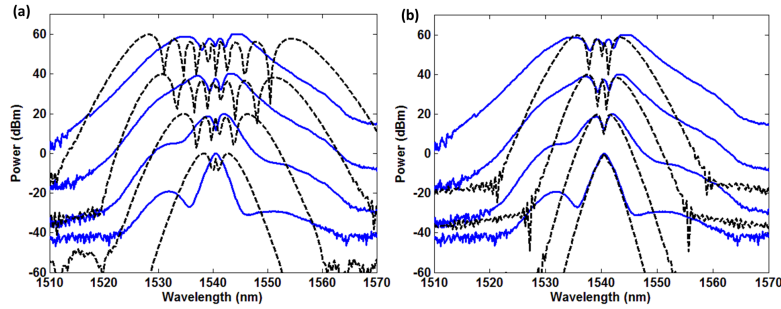
Figure 3.19 (a) The simulated (dotted black lines) and experimental (solid blue lines) for the Re(\gamma) of 475 W^{-1}m^{-1} for input peak powers of 4.9 W, 9.8 W, 22 W and 44 W respectively from bottom to top. (b) The comparison of the simulated and experimental SPM spectral with a reduced Re(\gamma) value of 150 W^{-1}m^{-1} .
