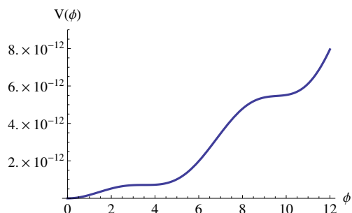
Figure 5. The axion inflation potential with f = 1.0 for the small field inflation (the field excursion \Delta\phi < 1 during the inflation).
