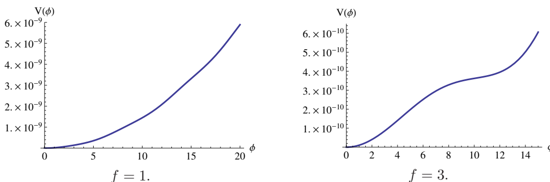
Figure 7. The axion inflation potential with a large axion decay constant for the large field inflation.
