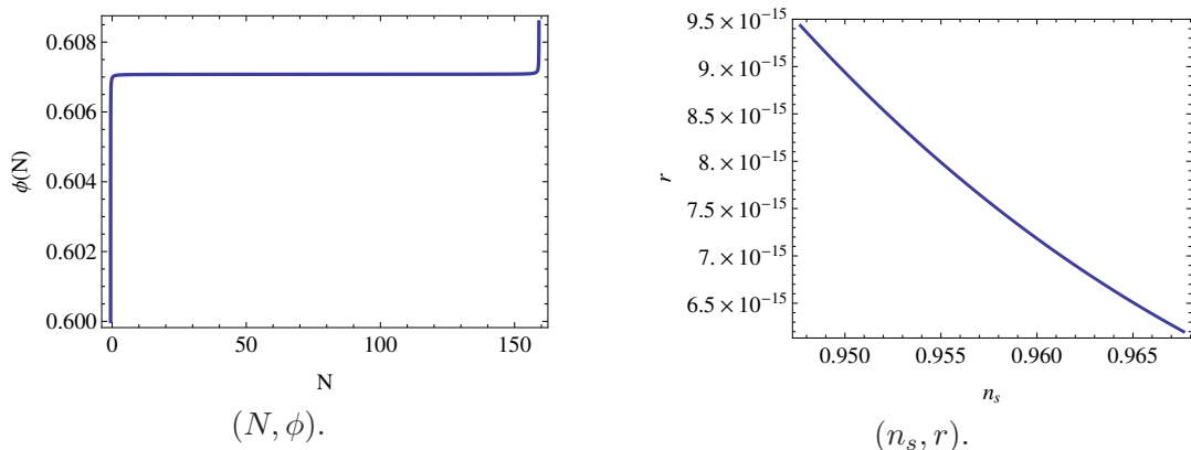
Figure 4. The inflaton amplitude as a function of the number of e-folds \phi(N) (Left) and (n_s, r) for N = [50, 60] (Right) for f = 0.01 , \Lambda_1/\Lambda_3 = 97 , and \Lambda_2/\Lambda_3 = 1 (corresponding to V_{\text{inf}}^{1/4}(N = 55) = 4.0 \times 10^{-6} ).
