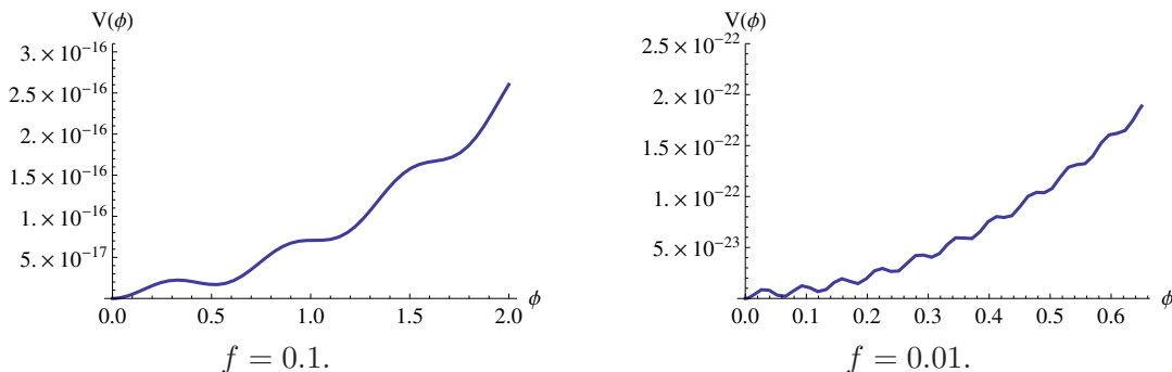
Figure 1. The axion inflation potentials with a sub-Planckian axion decay constant f = 0.1 (left) and f = 0.01 (right) for the small field inflation (the field excursion \Delta\phi < 1 during the inflation).
