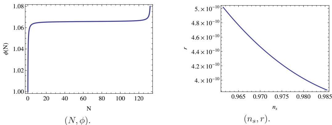
Figure 3. The inflaton amplitude as a function of the number of e-folds \phi(N) (Left) and (n_s, r) for N = [50, 60] (Right) for f = 0.1 , \Lambda_1/\Lambda_3 = 4.9 and \Lambda_2/\Lambda_3 = 0.25 (corresponding to V_{\text{inf}}^{1/4}(N = 55) = 6.1 \times 10^{-5} ).
