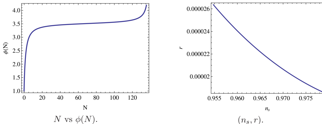
Figure 6. (The inflaton amplitude as a function of the number of e-folds \phi(N) (Left) and (n_s, r) for N = [50, 60] (Right) for f = 1.0 , \Lambda_1/\Lambda_3 = 1.0 and \Lambda_2/\Lambda_3 = 1.9 (corresponding to V_{\text{inf}}^{1/4}(N = 55) = 9.0 \times 10^{-4} ).
