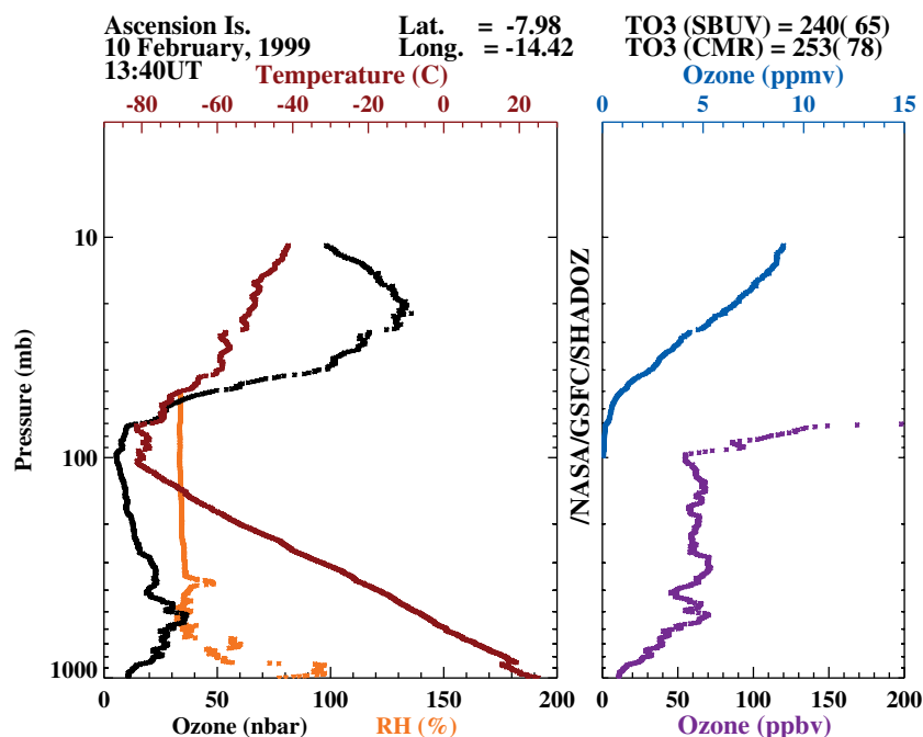
Figure 2. Typical profile from the website showing data in partial pressure (ozone, on left), relative humidity and temperature from radiosonde (also left), with ozone volume mixing ratio on right panel. Example is for an Ascension Island sounding on 10 February 1999. Reliability of humidity data above 500 hPa is highly variable station-to-station. Generally, images in the SHADOZ archive do not display useful data above 50 hPa.
