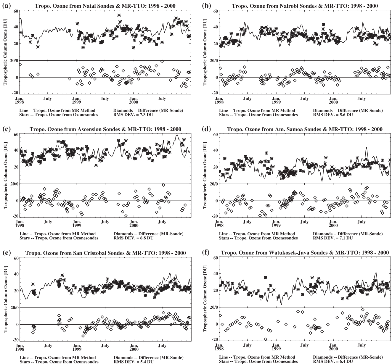
Figure 8. Integrated tropospheric ozone for six SHADOZ sites (*) with 9-day averaged tropospheric ozone for the corresponding location derived from TOMS by the modified-residual method [Thompson and Hudson, 1999]. Nine-day running averages of TOMS data are used to minimize equatorial data gaps, scan angle artifacts and aerosol effects. The modified-residual method is restricted to tropical air masses, which are defined as being within the zone of the wave-one feature in total ozone—usually at \pm 20^\circ from the equator. (A) Natal, (B) Nairobi, (C) Ascension, (D) Samoa, (E) San Cristóbal, (F) Watukosek. Lower panel displays percent differences from satellite reading.
