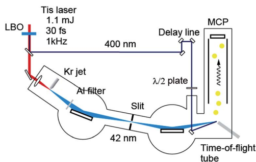
Fig. 2 Experimental setup for time-resolved photoelectron spectroscopy using high harmonic pulses. Ti is Ti:sapphire.
